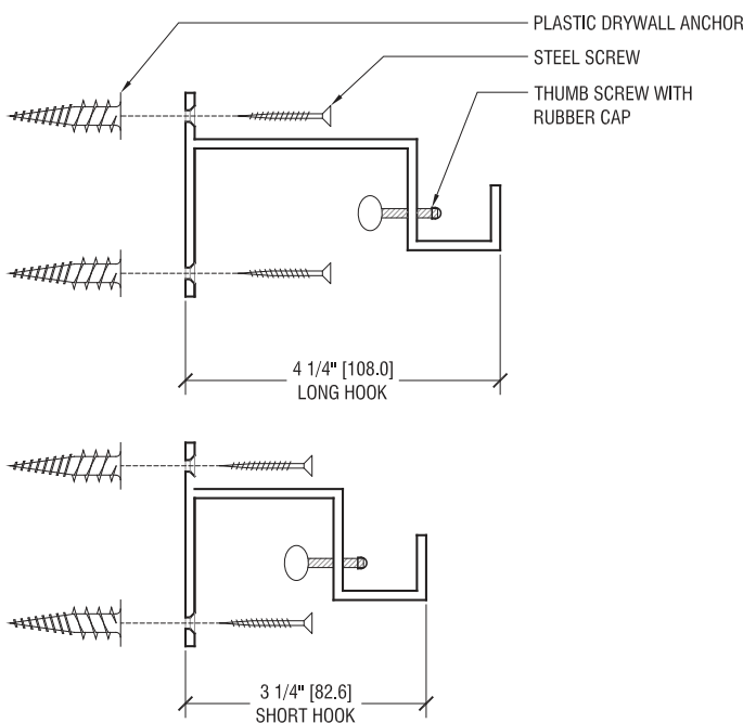
Figure 1. Pool wall-hook information
