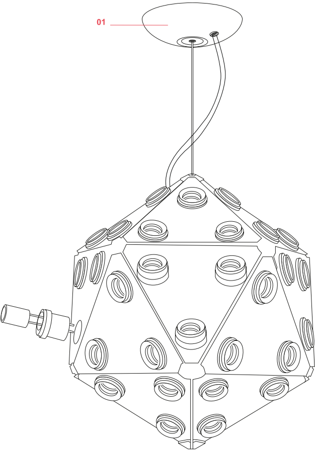
01. Rose assembly
